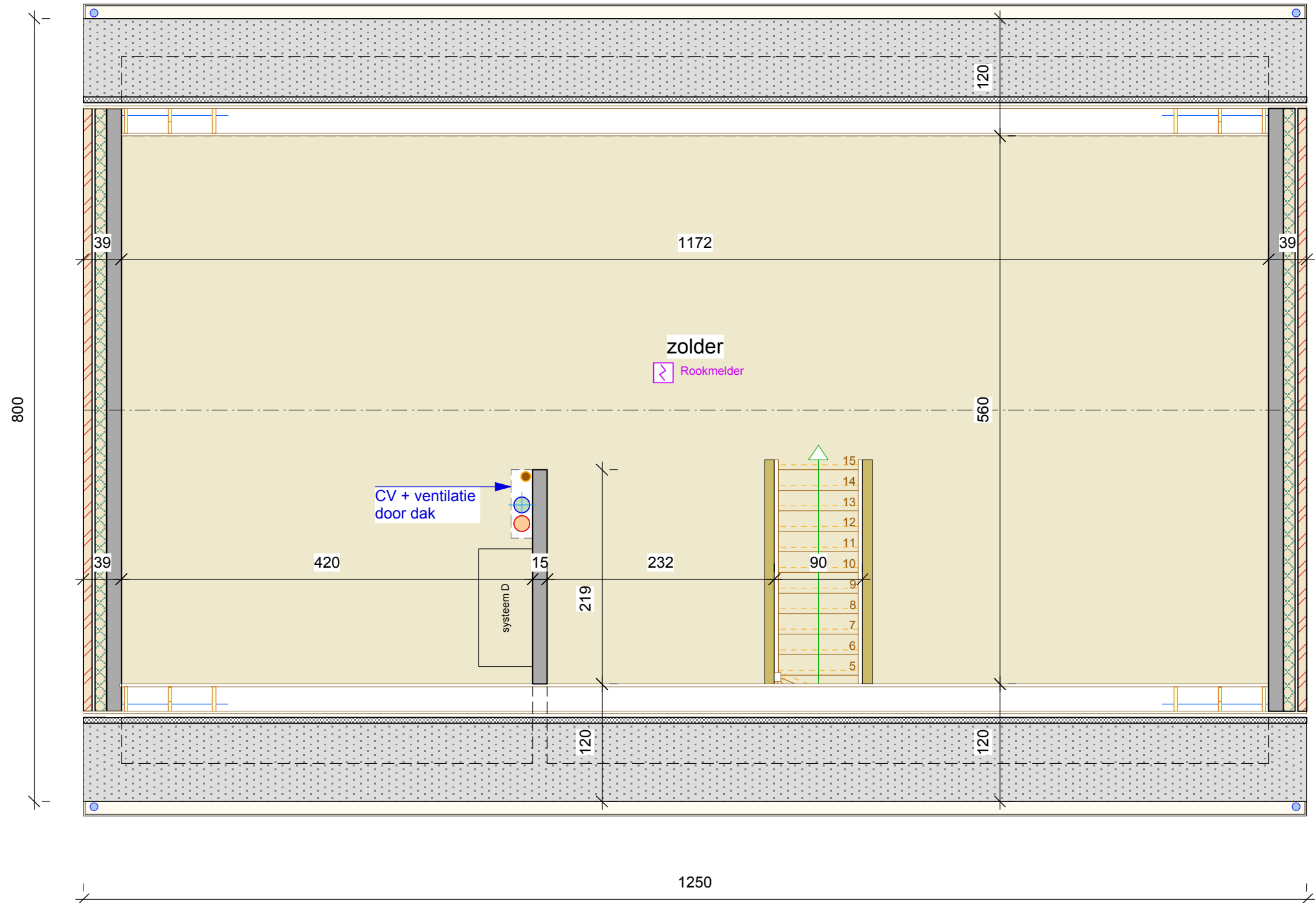
Plan ZOLDERVERDIEPING
